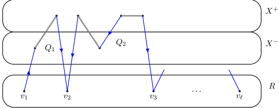
FIGURE 5. A copy of P in D[R \cup X] with startpoint v_1 and endpoint v_\ell that covers all the vertices in R , as found in Lemma 6.9. The section of the path between v_i and v_{i+1} is found by Lemma 6.8. The double edges indicate that both orientations are present, as found by applying the bipseudorandom property.
